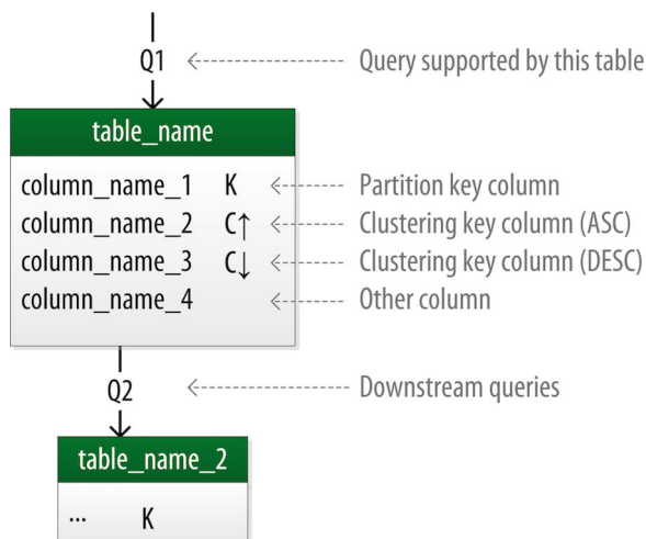
Figure 5-4. A Chebotko logical diagram
