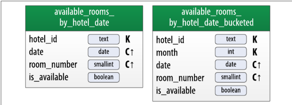
Figure 5-10. Adding a month bucket to the available_rooms_by_hotel_date table
